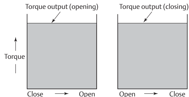
Figure 2. Double-Acting torque characteristic
