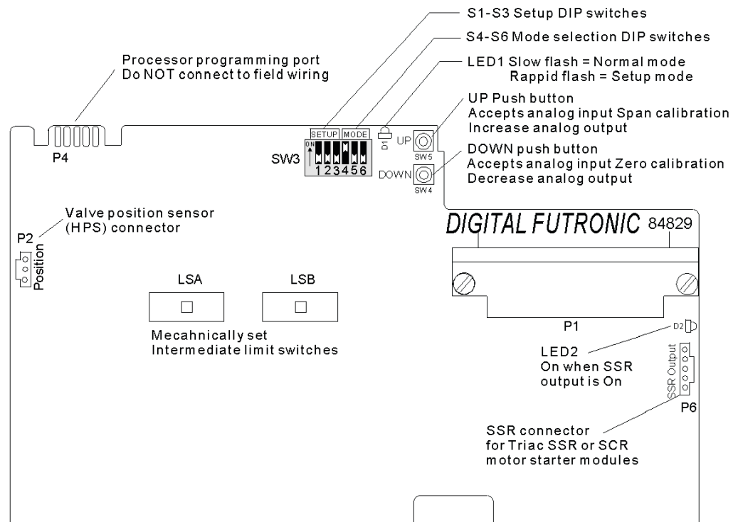
Figure 3 Locations of DIP switches and Push-buttons
