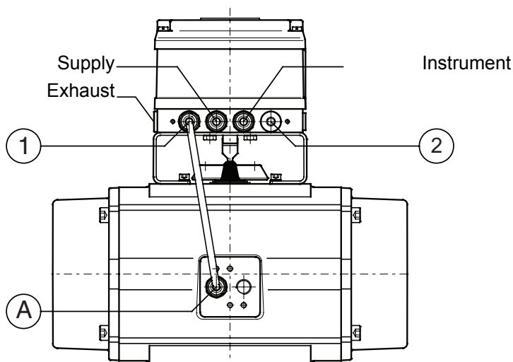
Pneumatic Connections Single acting
