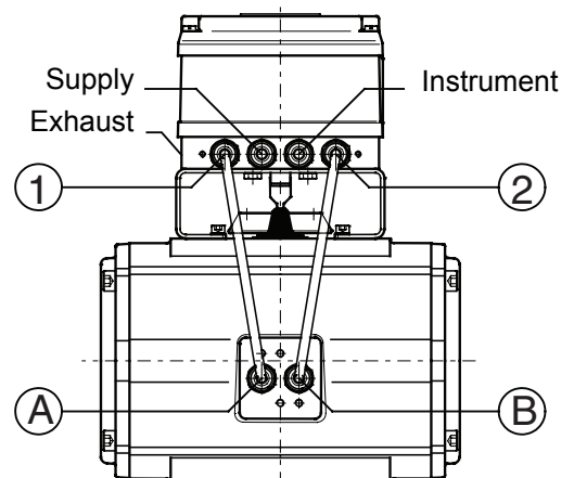
Pneumatic connections
